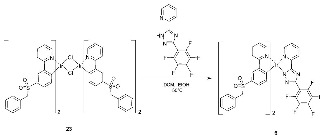
Scheme 5. Synthetic route for complex 6.
