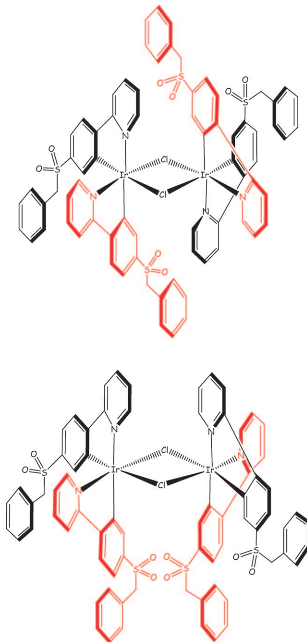
Scheme 7. Alternative cis chiral arrangements of the dichloro-bridged dimer 25 .
