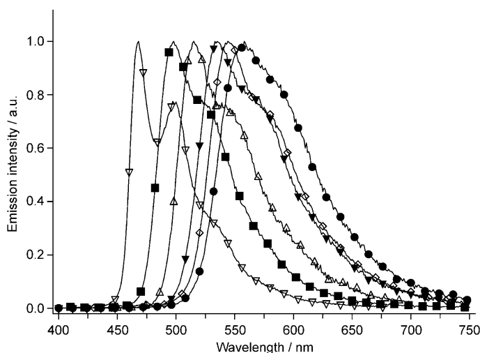
Figure 3. Normalised RT emission spectra of complexes 1–6 recorded in \text{CH}_2\text{Cl}_2 ( \lambda_{\text{ex}}=350 \text{ nm} ). \diamond : 1 , \blacksquare : 2 , \bullet : 3 , \blacktriangledown : 4 , \triangle : 5 , \nabla : 6 .
