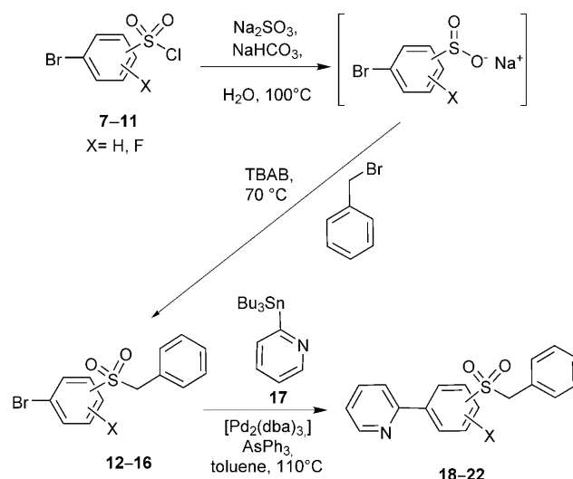
Scheme 2. General procedure for the synthesis of ligands 18–22 ; dba = dibenzylideneacetone, TBAB = tetra- N -butyl ammonium bromide.
