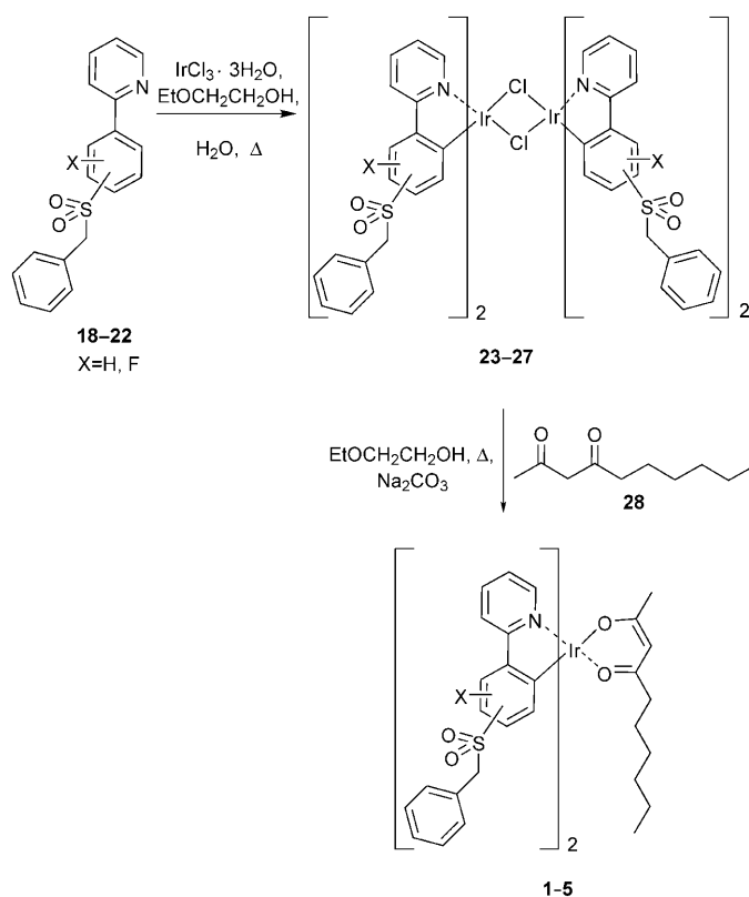
Scheme 3. General procedure for the synthesis of the iridium complexes 1–5.
