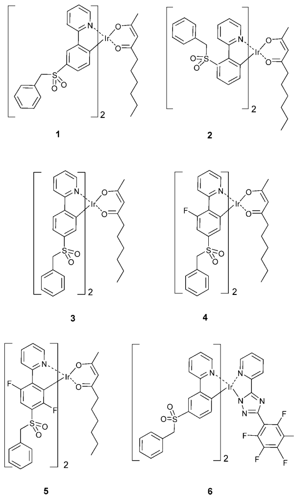
Scheme 1. Schematic formulas and numbering of the synthesised iridium complexes.
