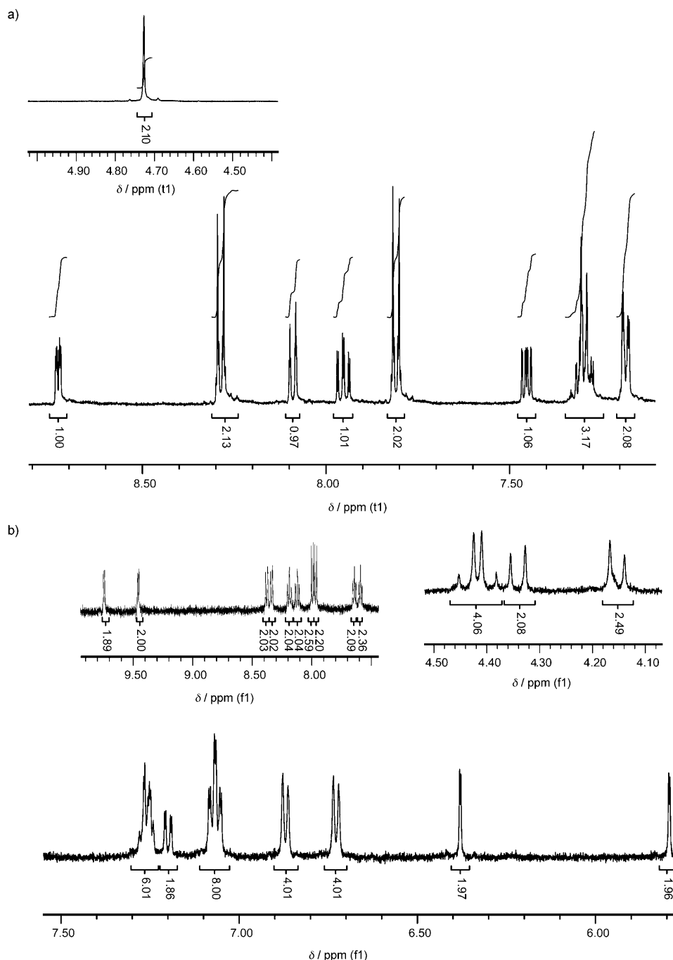
Figure 1. a) ^1\text{H} NMR spectrum of cyclometalating ligand 20 in [\text{D}_6]\text{DMSO} ; b) ^1\text{H} NMR spectrum of dichloro-bridged dimer 25 in [\text{D}_6]\text{DMSO} .
