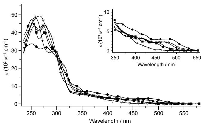
Figure 2. Absorption spectra of complexes 1–6 recorded in \text{CH}_2\text{Cl}_2 at RT. The inset shows a magnified view of the spectra between \lambda=350 and 550 \text{ nm} . \diamond : 1 , \blacksquare : 2 , \bullet : 3 , \blacktriangledown : 4 , \triangle : 5 , \nabla : 6 .
