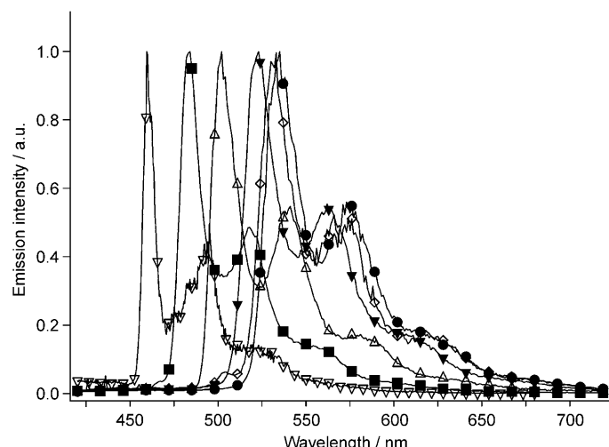
Figure 4. Normalised emission spectra of complexes 1–6 measured at 77 K ( \lambda_{\text{ex}}=350 nm) in butyronitrile glass matrix. \diamond : 1 , \blacksquare : 2 , \bullet : 3 , \blacktriangledown : 4 , \triangle : 5 , \nabla : 6 .
