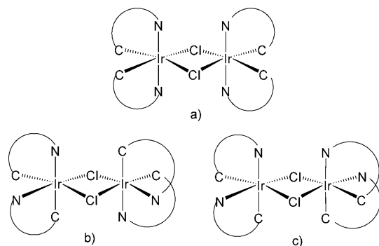
Scheme 6. Schematic representation of the stereochemistry of the dichloro-bridged iridium dimer complexes: a) trans arrangement reported in the literature; [6a,b,16] b) and c) cis chiral arrangements.
